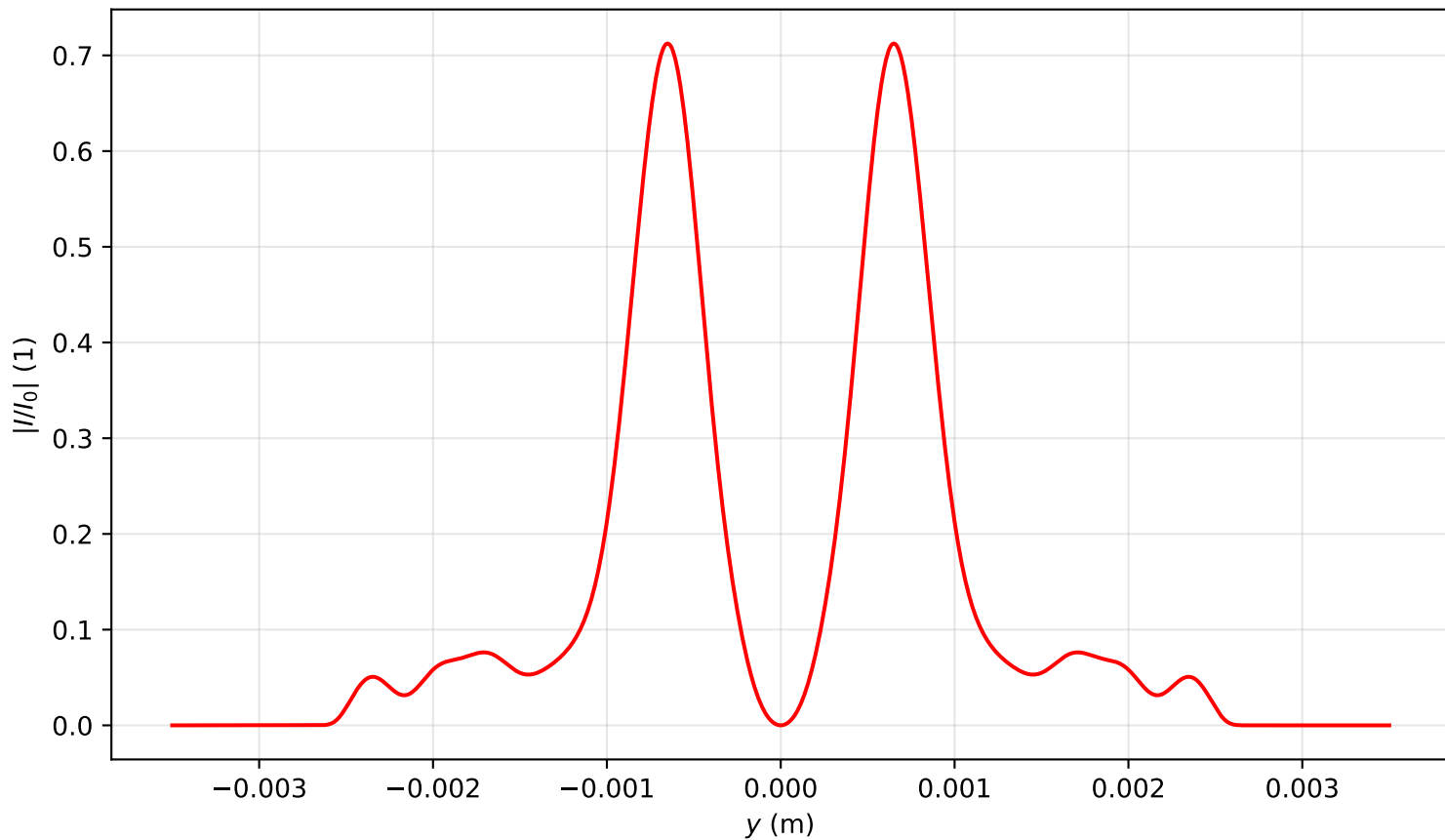
Intensity profile I(x = 0, y, z = 3.184)/I_0 , P_{in}=5.0P_{cr} , artificial time
